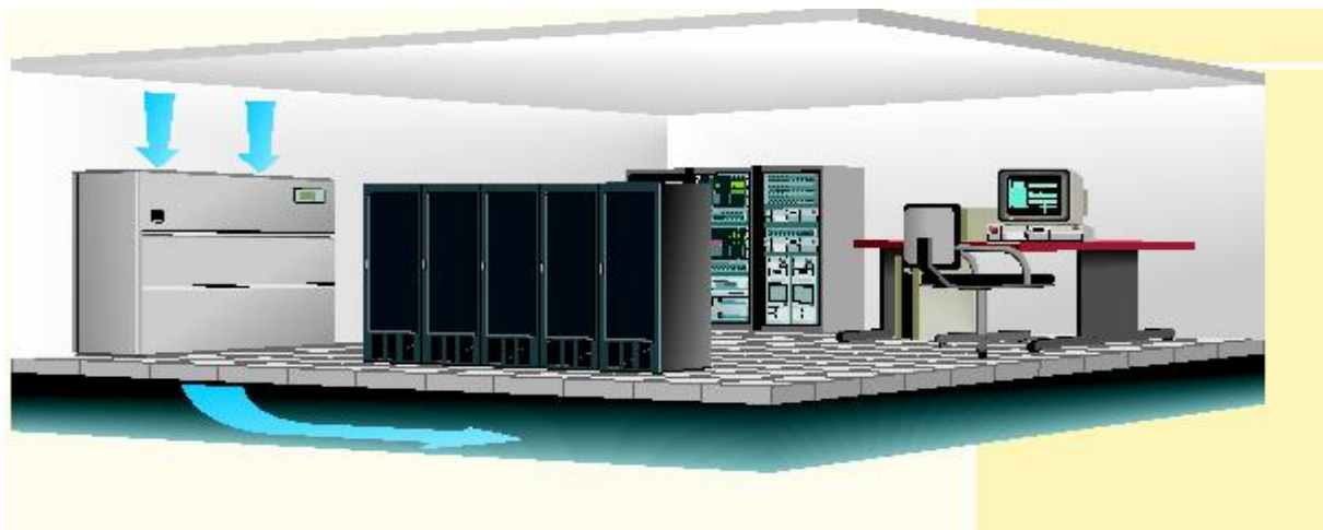
CRAC Airflow Pattern
